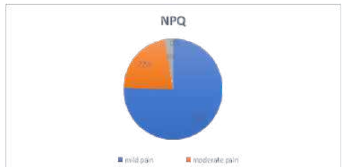
Figure 2: NPQ.
